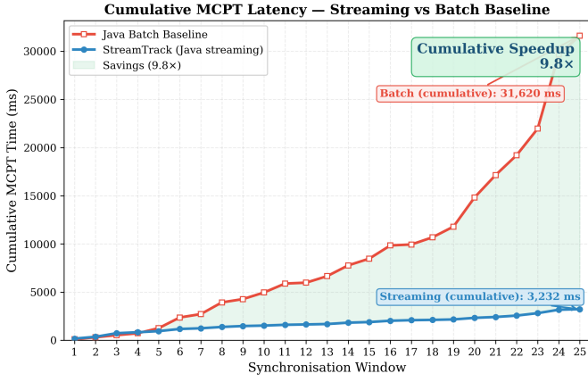
Fig. 4. Cumulative MCPT latency across 25 consecutive windows on the Woven WTS dataset (4 cameras). Incremental streaming achieves a 9.8× speedup over the batch baseline by eliminating redundant state recomputation.
